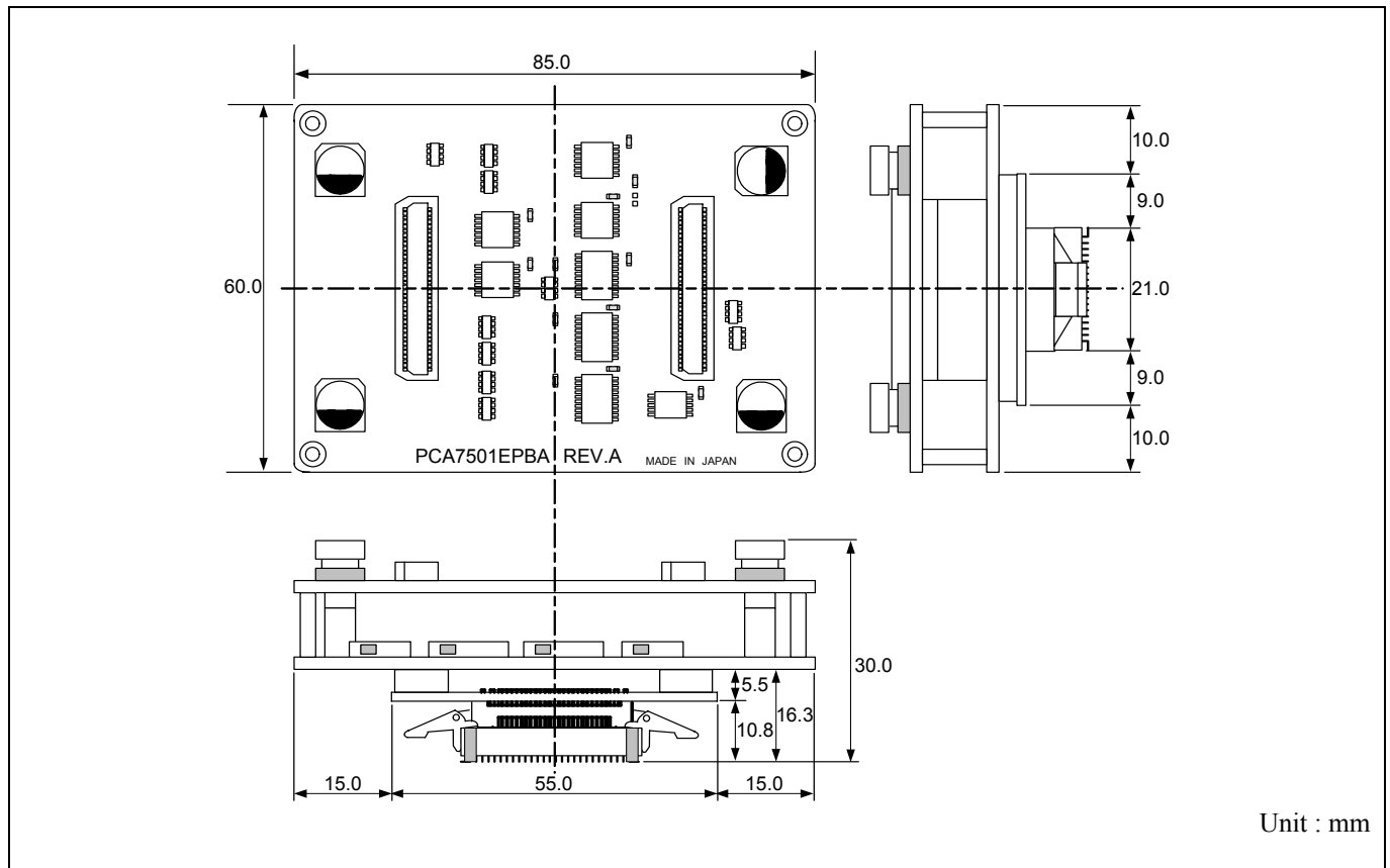
Figure 4.3 External dimensions of the emulation probe
